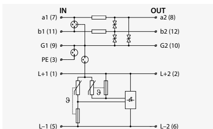
DMP-012-V/1-FR1 (see Figures. 47, 48)
