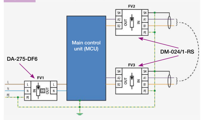
Fig. 43a Version for loop current up to 500 mA
