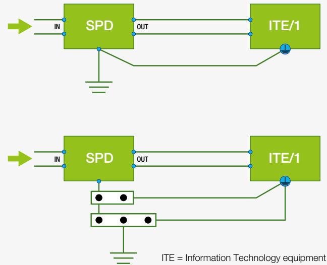
Fig. 17 Correct connection
