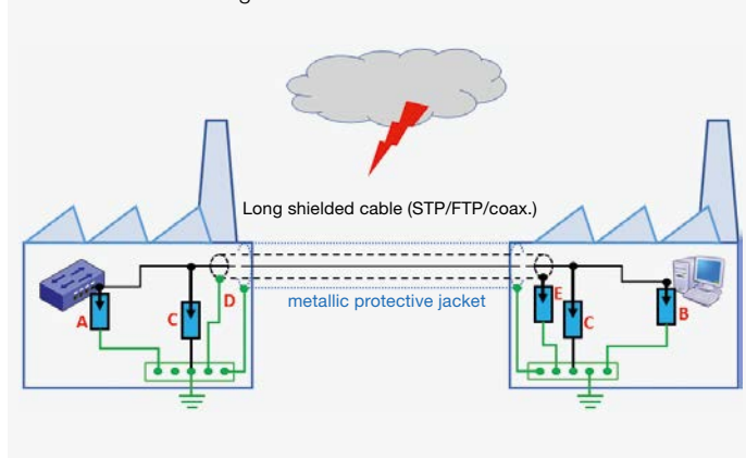
Fig. 55 Earthing of a long shielded cable / bundle / cable duct / cable trough
