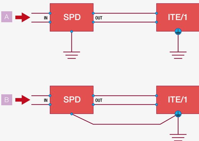
Fig. 16 Incorrect protective ground connection
