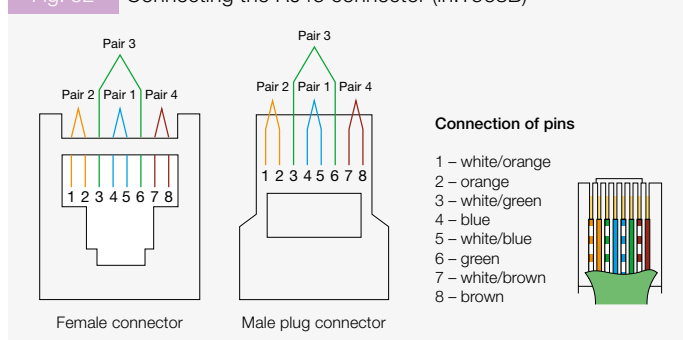
Fig. 52 Connecting the RJ45 connector (in.T568B)
