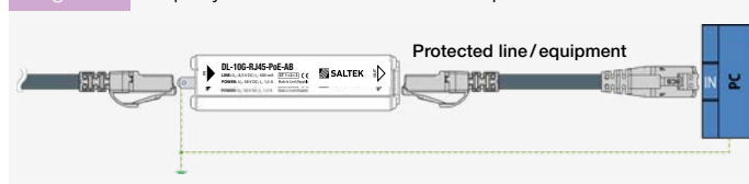
Fig. 56 Properly oriented SPD for efficient protection
