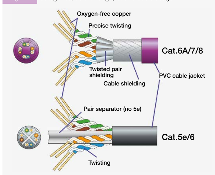
Fig. 51 Categories, data throughput and cable usage
