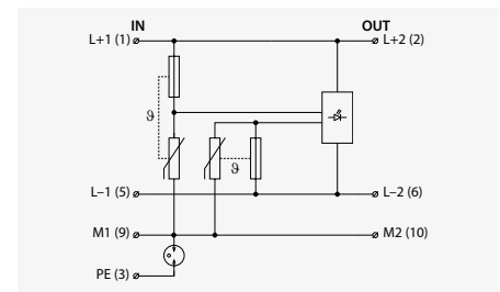
DP-024-V/1-F16 (see Fig. 32)
