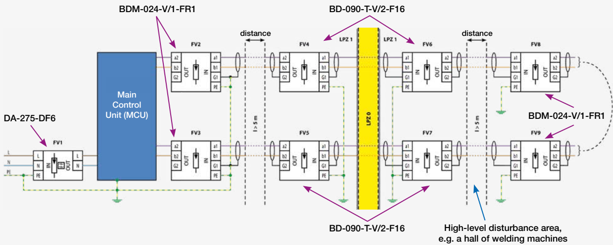
Fig. 46 RS-232 line protection (e.g., DSI programming)
