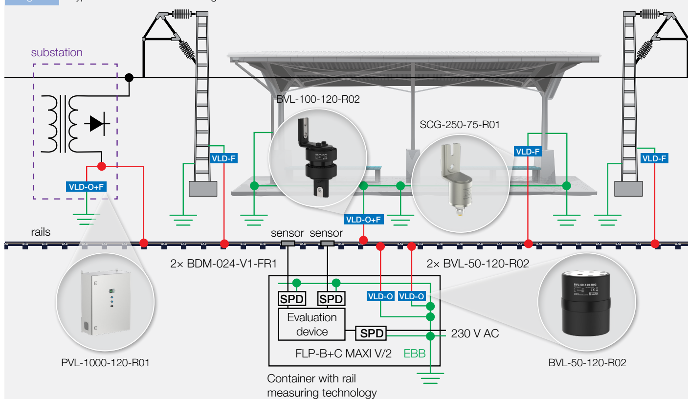
Fig. 2 Typical installation of VLDs along the railroad.
