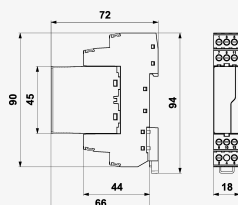
Product dimensions
