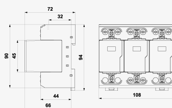
Product dimensions
