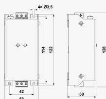
Product dimensions
